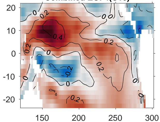
Combined EOF4(U10)
