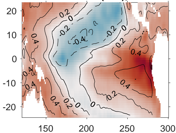
Combined EOF3(SST); cf=0.08
