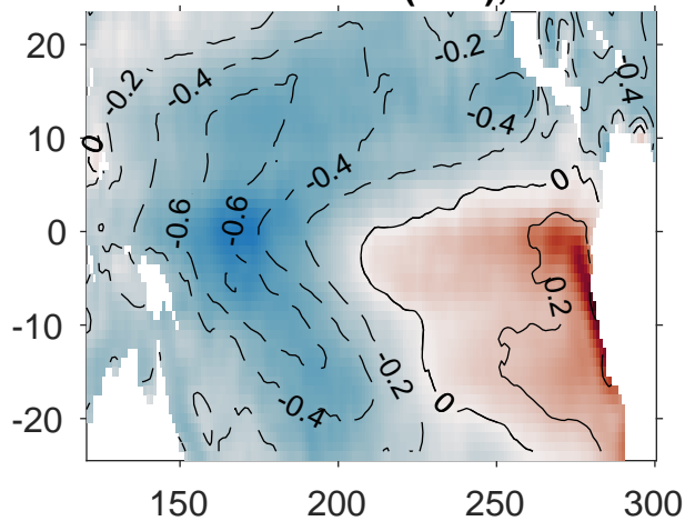
Combined EOF2(SST); cf=0.1
