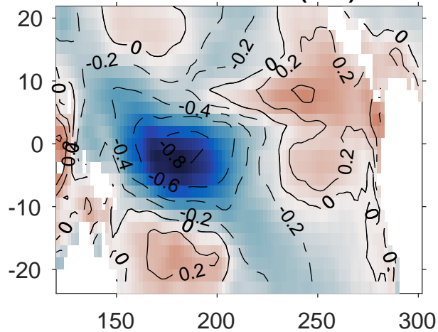
Combined EOF1(U10)
