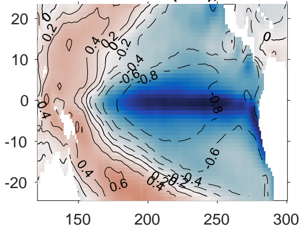
Combined EOF1(SST); cf=0.25
